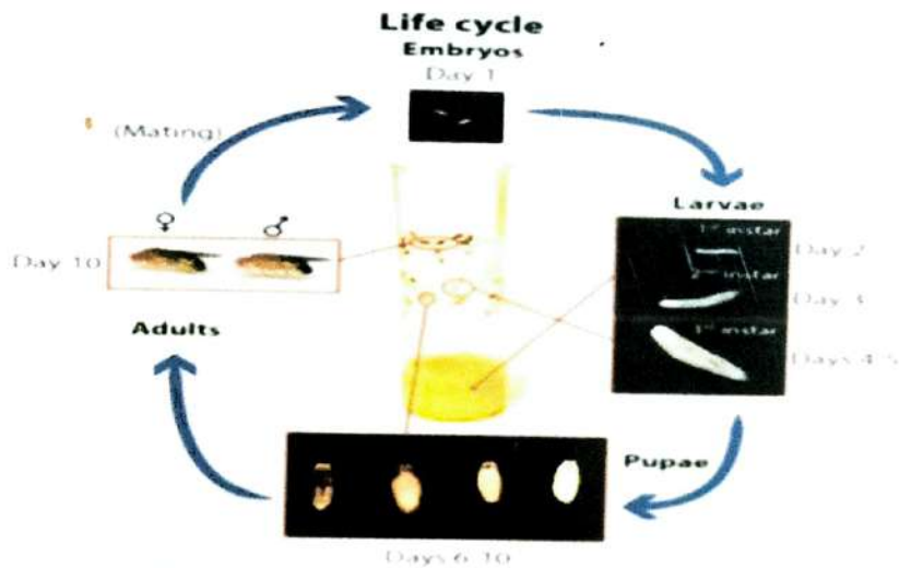
Figure. The image shows the complete cycle of Drosophila cultured in a vial in the lab
