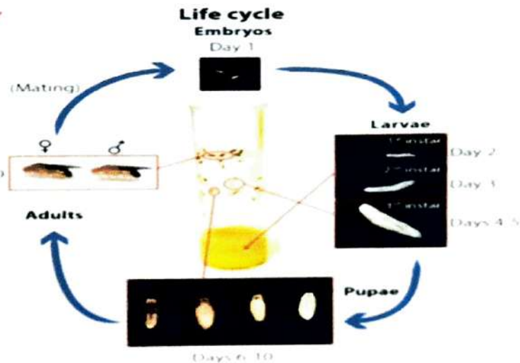
Figure: The image shows the complete cycle of Drosophila cultured in a vial in the lab
