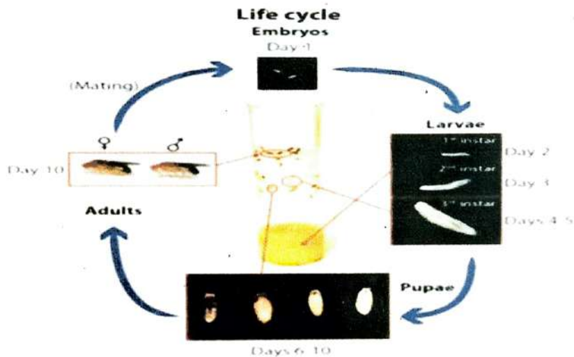
Figure. The image shows the complete cycle of Drosophila cultured in a vial in the lab
